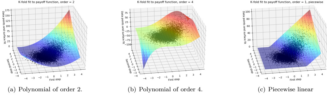
FIGURE 4. StackMC variance reduction on an Asian option with M = 2 .
